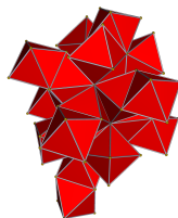
24-cell
