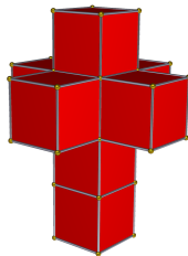
Tesseract
