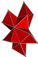
16-cell
