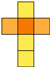
Cube
