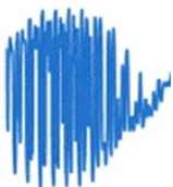
Speech synthesis
